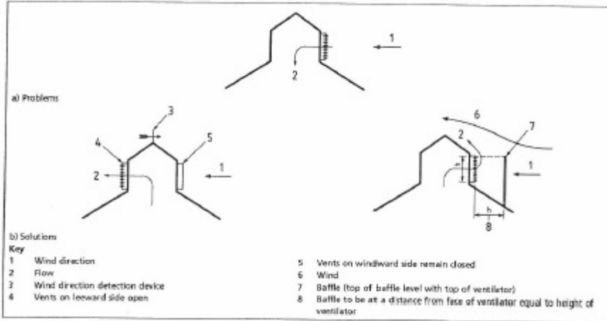
Figure D.2 Louvered ventilators installed in the vertical
